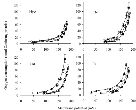
Figure 5 Effect of superoxide plus palmitate in the absence (black triangle) or presence (open circle) of GDP on basal proton conductance (black square) of red gastrocnemius muscle mitochondria isolated from thermoneutral controls (TN), cold-acclimated (CA), hypothyroid (hypo) or T_3 -treated ducklings. Proton conductance was assessed by simultaneous measurement of membrane potential and oxygen consumption. Superoxide generation was obtained by addition of 50 \mu M xanthine (X) and 8 mU/3.5 mL xanthine oxidase (XO). When observed, increase in proton conductance was reversed by 1 mM GDP. All measurements were conducted with 5 mM succinate as substrate, 5 \mu M rotenone, 1 \mu g/mL oligomycin, 65 ng/mL nigericin, 0.3% FAF-BSA and 25 \mu M palmitate. Mitochondria from CA or T_3 -treated ducklings showed a much larger GDP sensitive XXO-activated proton conductance compared with TN or hypothyroid birds in which XXO had no major effect. Data are means \pm S.E.M. from 5 to 11 independent determinations.
